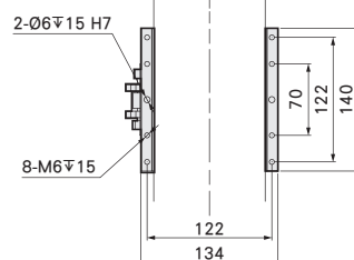
B-Detail View
