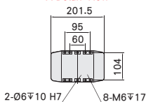
A-Detail View
