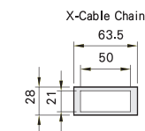
A-Detail View
