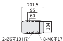
A-Detail View
