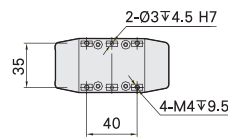
A-Detail View
