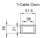
C-Detail View
