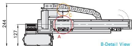
B-Detail View
