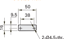
C-Detail View
