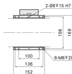
B-Detail View
