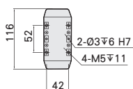
A-Detail View
