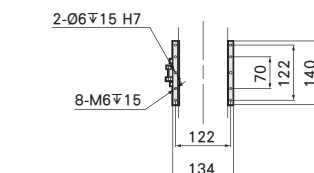
C-Detail View
