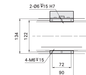
B-Detail View
