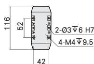
A-Detail View
