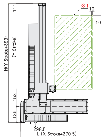
C View
