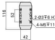
A-Detail View
