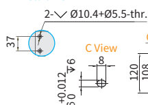
B-Detail View
