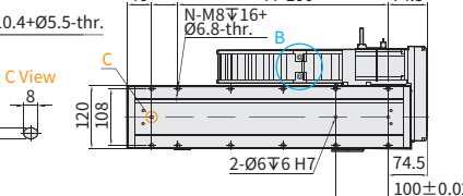
C View
