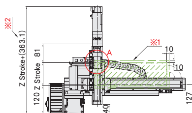
B-Detail View
