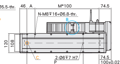
C View
